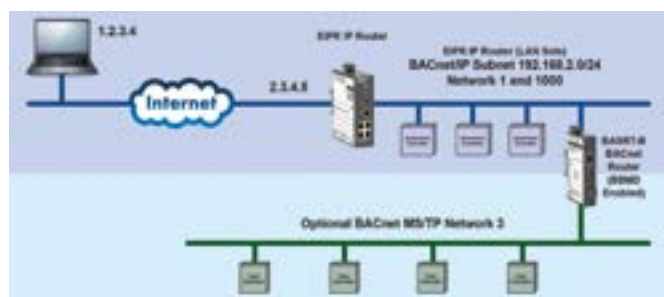
Figure 2: Remote Access to BACnet Network
