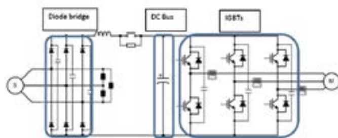
VFD topology
