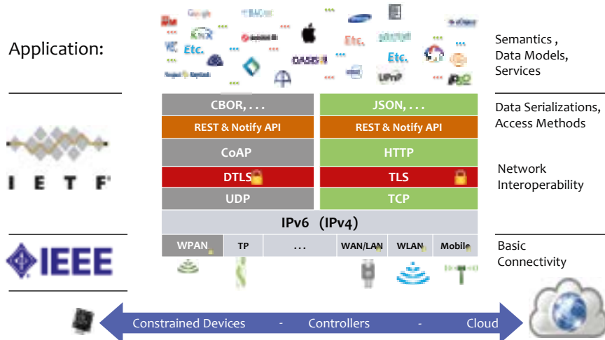
Fig 2: Typical IoT Technology Stacks
