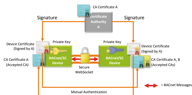
Figure 2: BACnet/SC Device Configuration for Secure WebSockets
