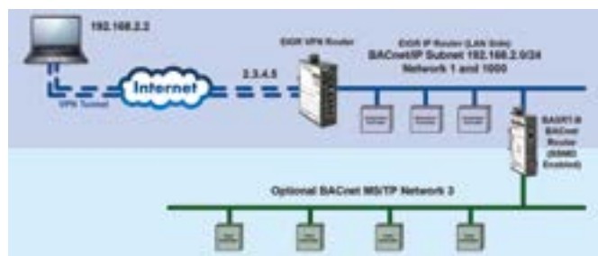
In the setup shown in Figure 3, a VPN router supporting bridging is used. The PC running the VPN client software connects to the VPN router establishing a secure VPN tunnel between the PC and the router. The PC is assigned an additional virtual interface with an IP address belonging to the 192.168.2.0/24 subnet, which is the same subnet as the existing BACnet network. Since all communication now occurs over the same subnet and VPN bridges pass all traffic through them, it greatly simplifies the setup by eliminating the use of BBMD.
