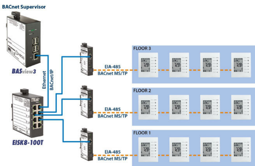
BACnet MS/TP Thermostat Network ©Contemporary Controls
