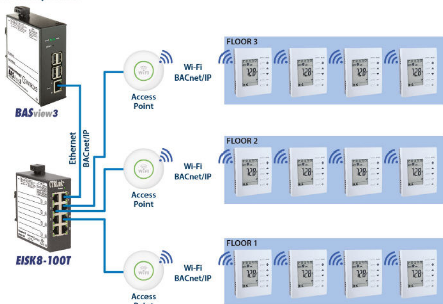
BACnet/IP Wi-Fi Thermostat Network ©Contemporary Controls
