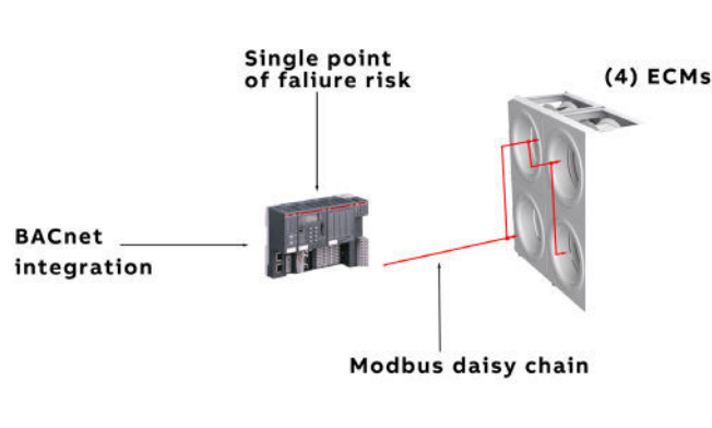
Figure 4: ECM fan array integration
